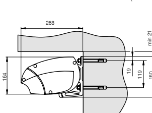
Wall/face mounting
