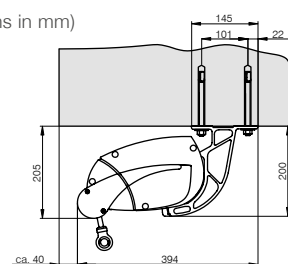
Ceiling/top mounting with a Variovalance
